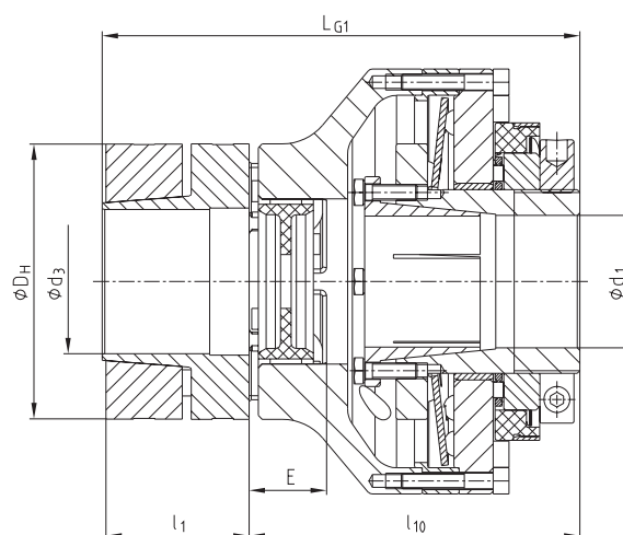
Hub type 4.5
