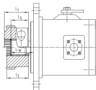
Clamping hub
