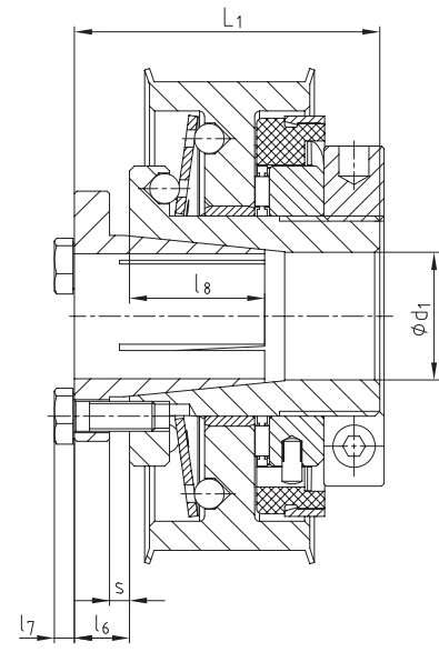
Hub type 4.5
