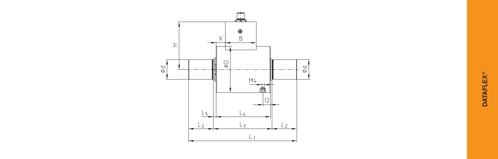
Combination of DATAFLEX® 32 with RADEX®-N
