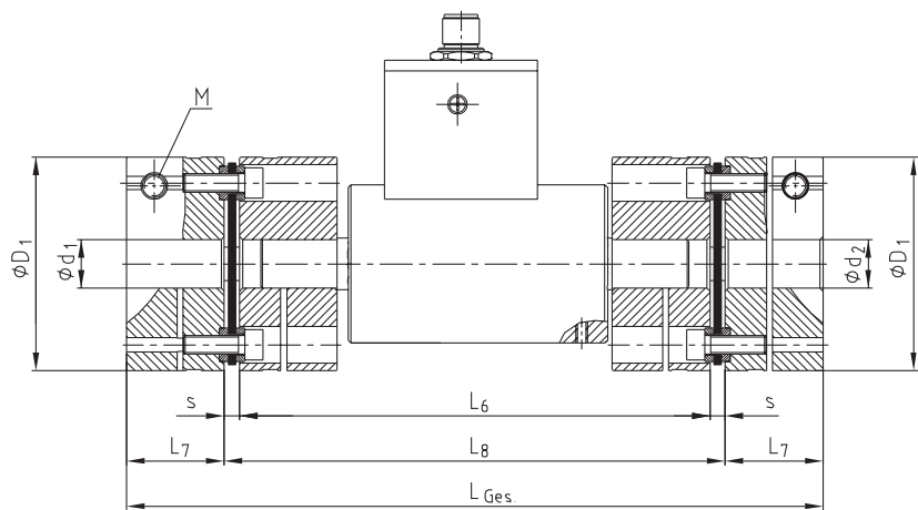
Combination of DATAFLEX® 16 with RADEX®-NC
