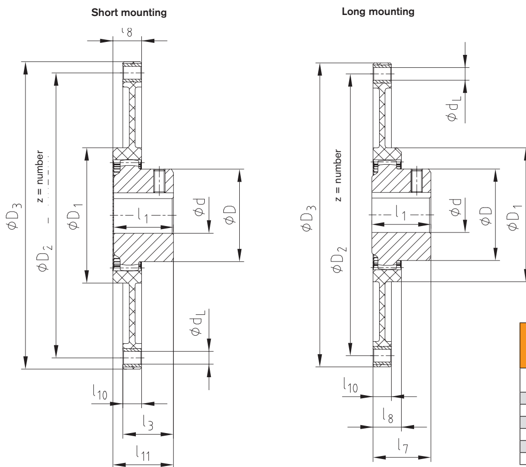
Flange dimensions acc. to SAE J 620 [mm]
