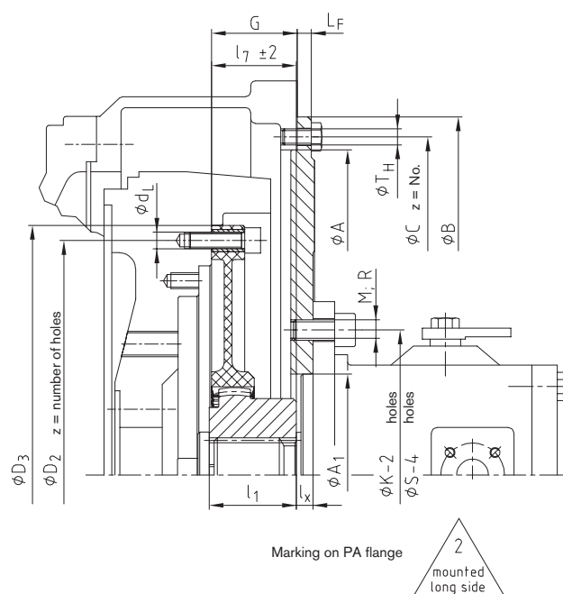
Long mounting of coupling (I7)
