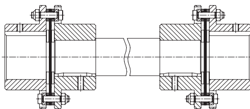
Type NNZ (see page 171)
