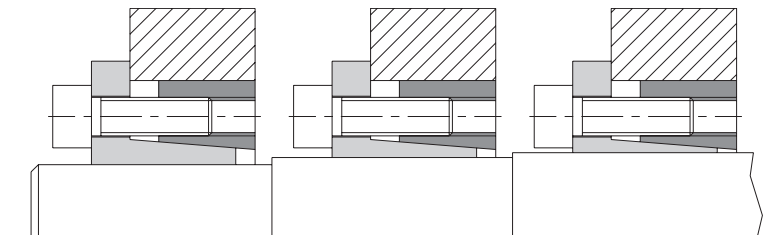
To fasten one size of hub on different shaft diameters
