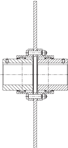
Type with brake disk
