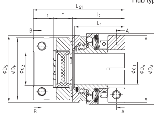
Hub type 6.1
