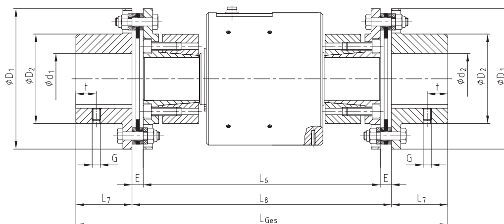
Combination of DATAFLEX® 85 with RADEX®-N
