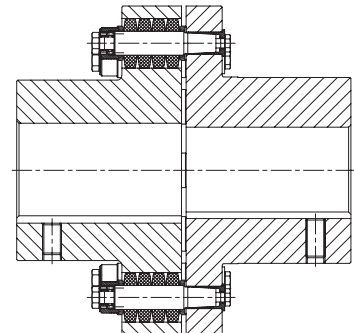
Backlash-free type
