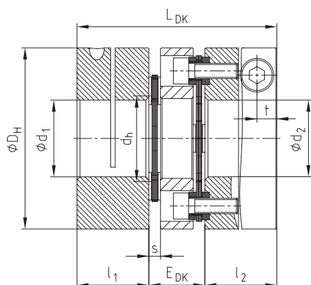
RADEX®-NC Types DK and EK Hub and spacer material aluminium (size 42 steel)/laminas stainless steel
