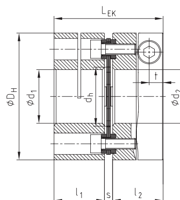
RADEX®-NC Types DK and EK Hub and spacer material aluminium (size 42 steel)/laminas stainless steel
