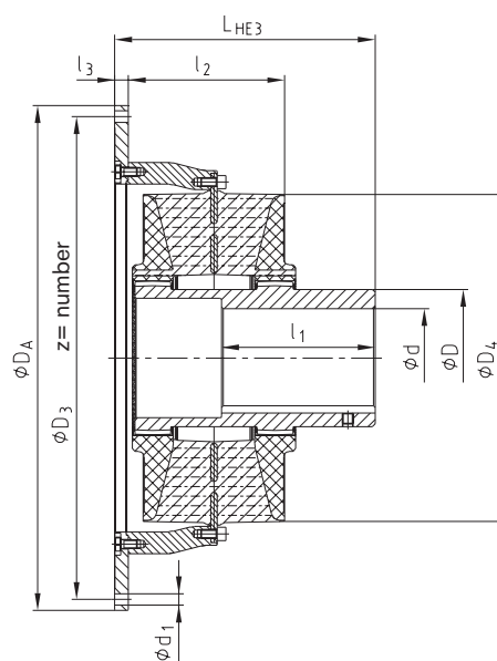
Flange dimensions acc. to SAE J 620 [mm]
