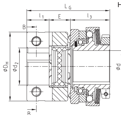
Hub type 2.9
